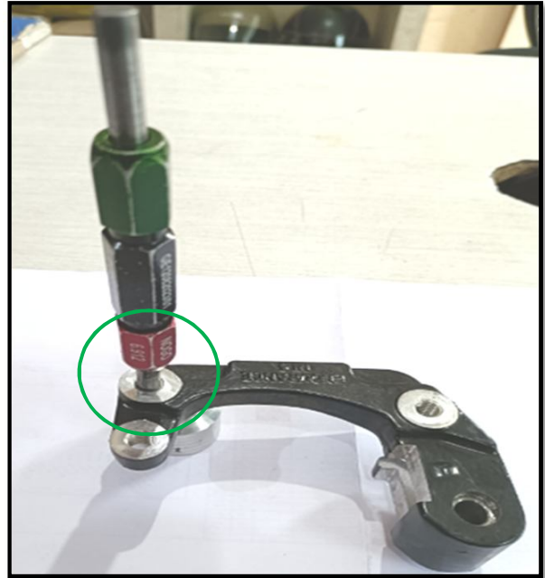
M8*1.25 Tapping PPG nogo side not passed.
